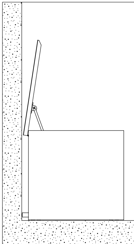
Distanzhalter max. Einstellung, ohne Wandsockel Spacer, maximum depth, use on walls without skirting boards
